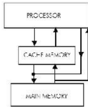
Figure 7.4: Cache Memory
